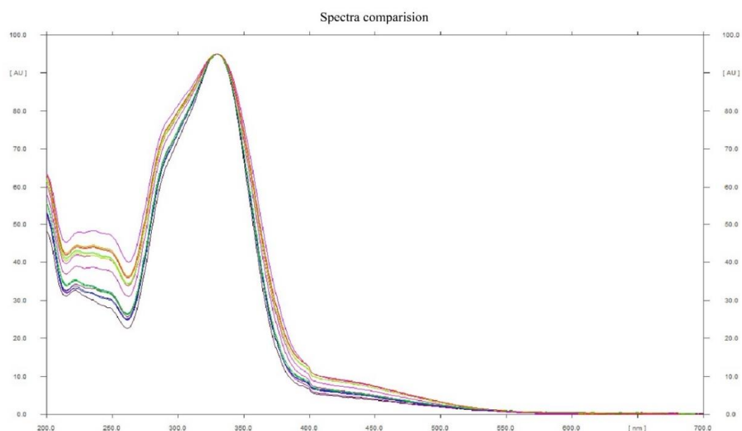
Figure 3 Peak identity determination by comparison of the absorbance spectra of rosmarinic acid among samples and standard rosmarinic acid
